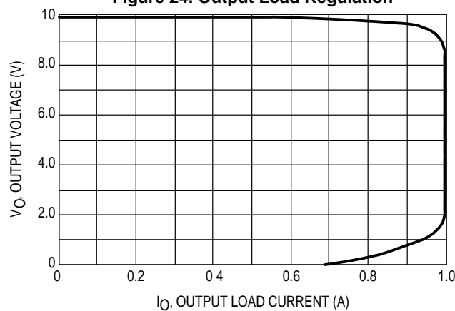
Figure 24. Output Load Regulation
