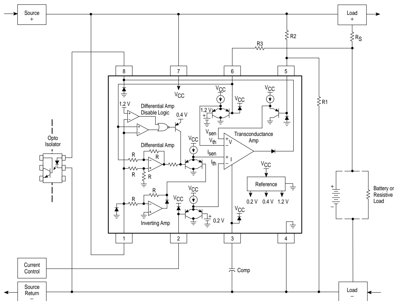
Figure 18. Load High-Side Current Sensing with Externally Adjustable Current and Internally Fixed Voltage Thresholds
