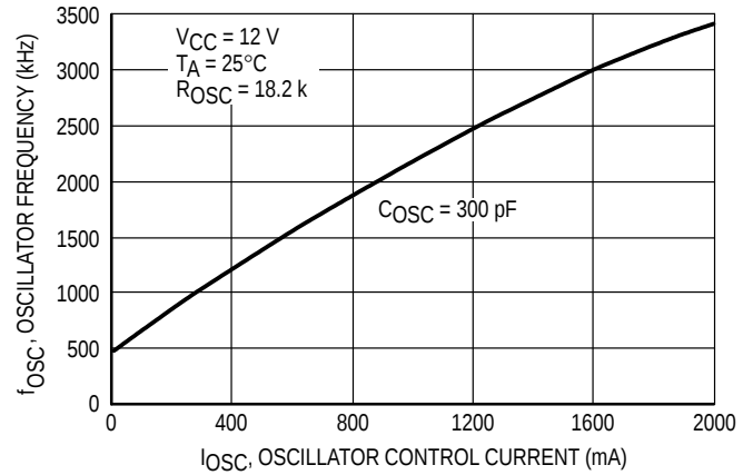
Figure 2. Oscillator Frequency versus Oscillator Control Current
