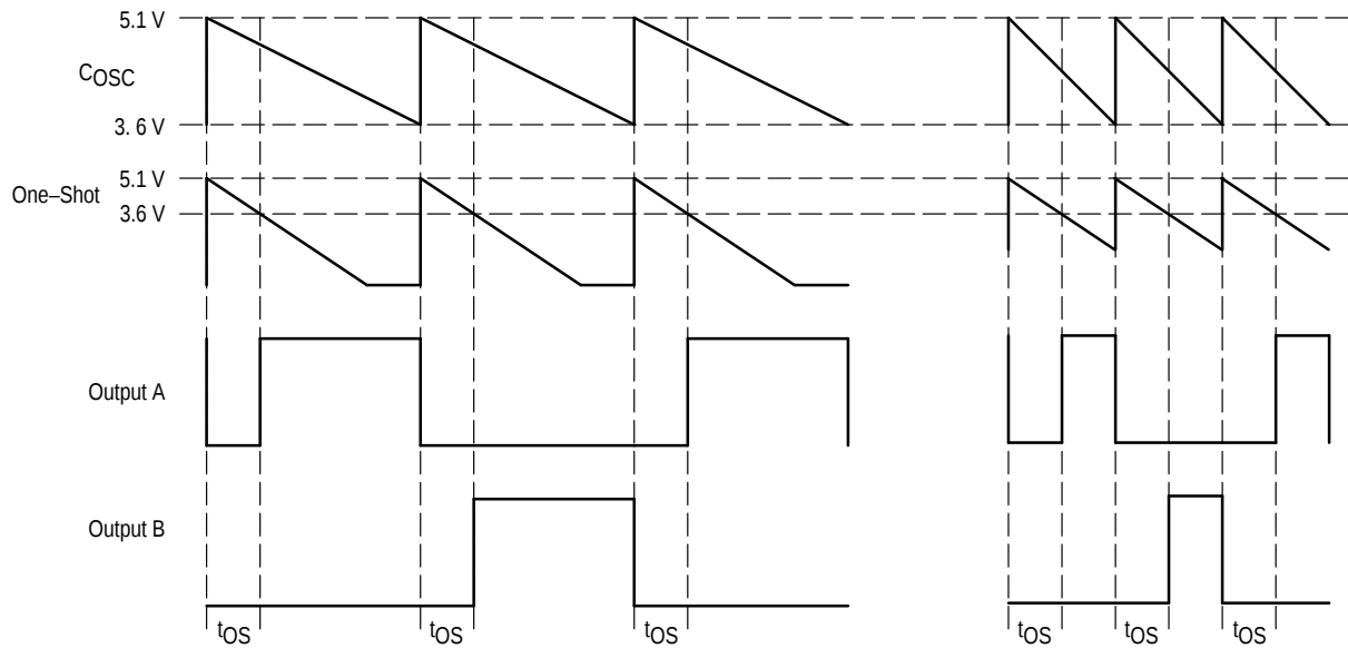
Timing Diagram
