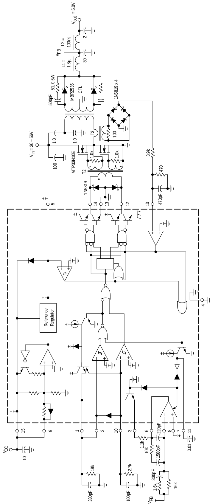
Figure 20. Application Circuit
