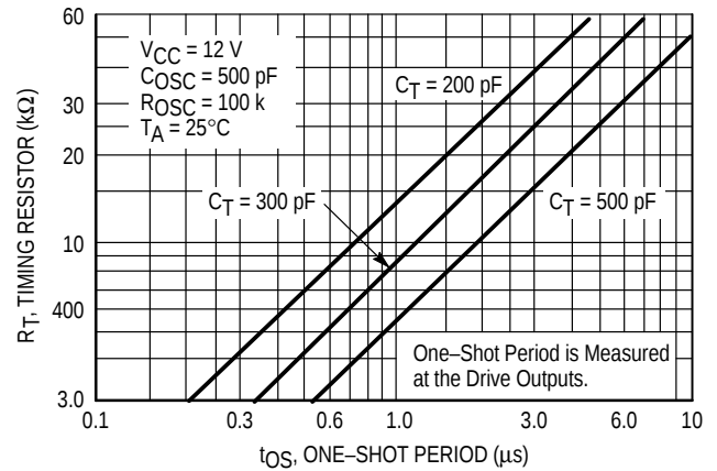
Figure 4. One-Shot Timing Resistor versus Period
